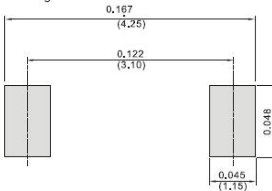
Fig.5 TYPICAL CAPACITANCE
